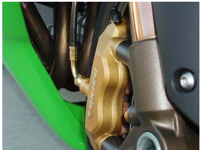
Picture C-2: Right caliper, notice fitting position
