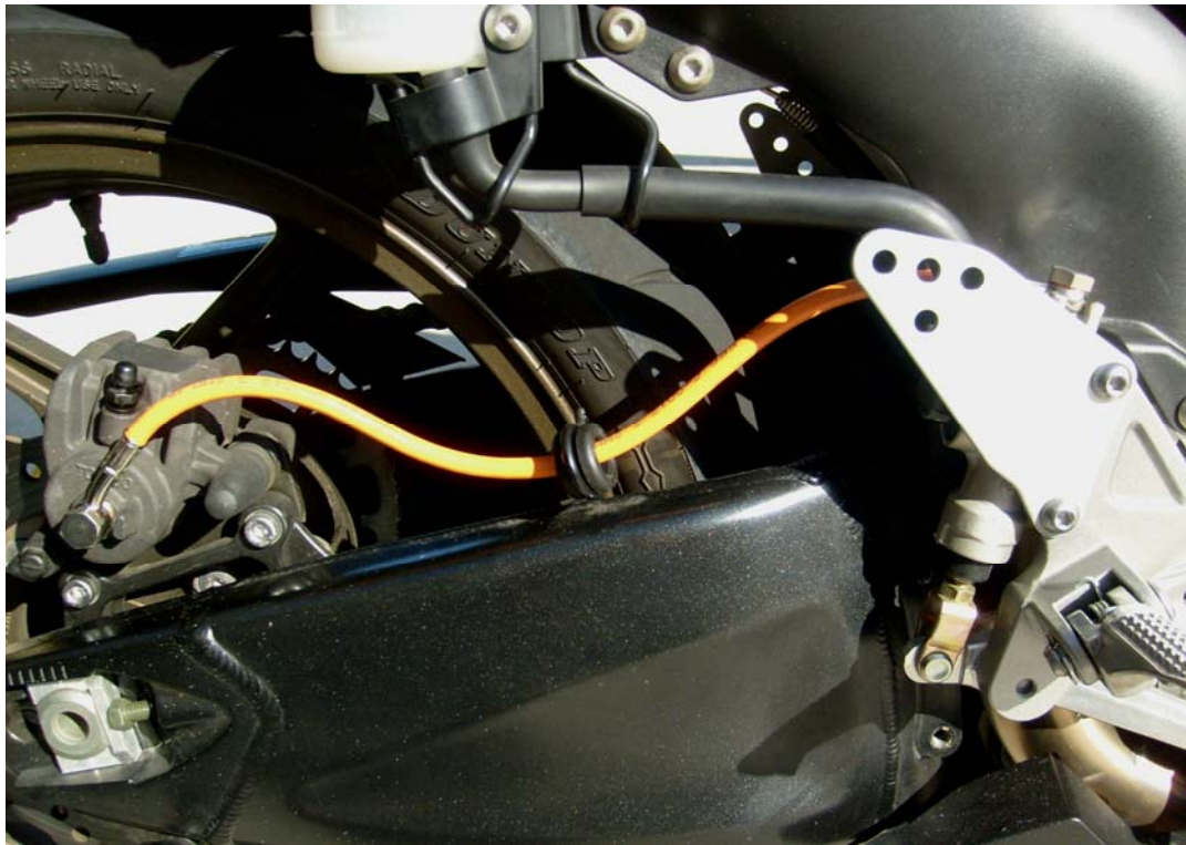
c. Rear Galfer line overall
