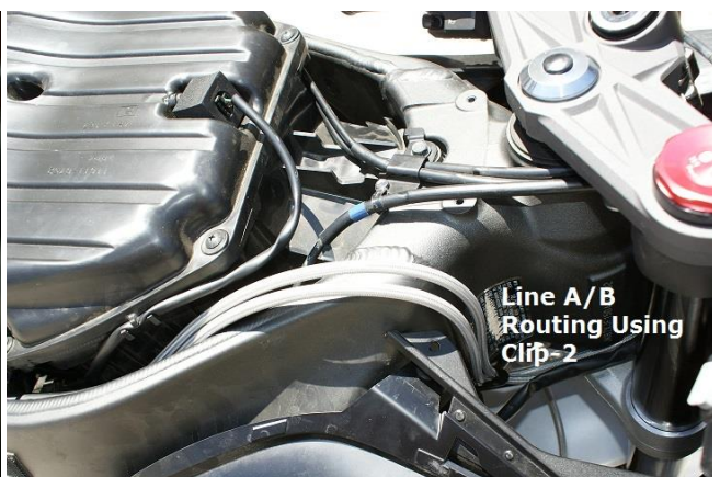
Picture 4 – Lines A & B Routing with Clip-2
