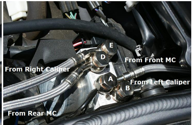
Picture 8 – ABS Unit
