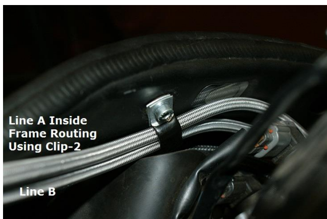
Picture 3 – Lines A & B Routing Inside Frame
